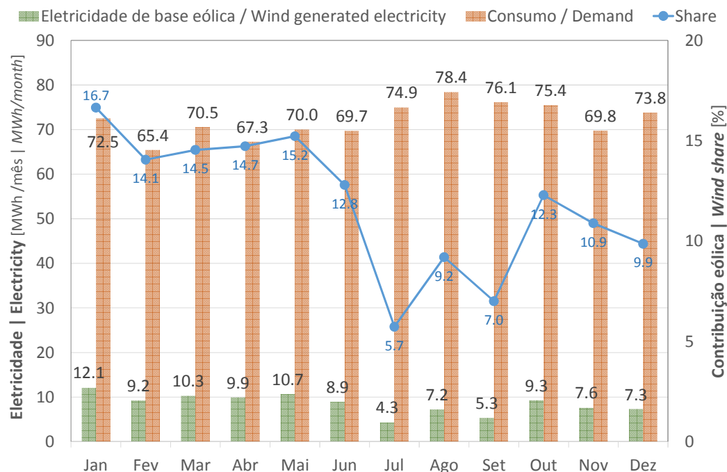
Figure 10: Wind generation vs. Electricity demand 2019 - Madeira Autonomous Region
