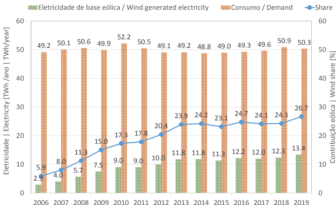
Figure 7: Wind generation vs. Electricity demand 2006-2019 - Mainland Portugal 2
