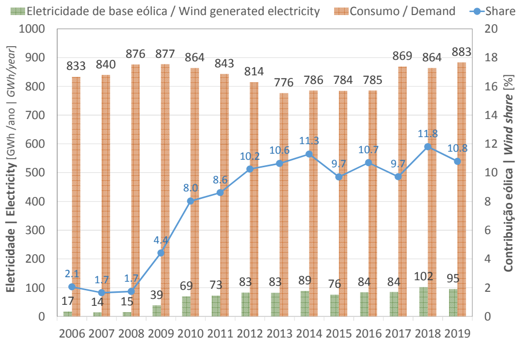
Figure 9: Wind generation vs. Electricity demand 2006-2019 - Madeira Autonomous Region
