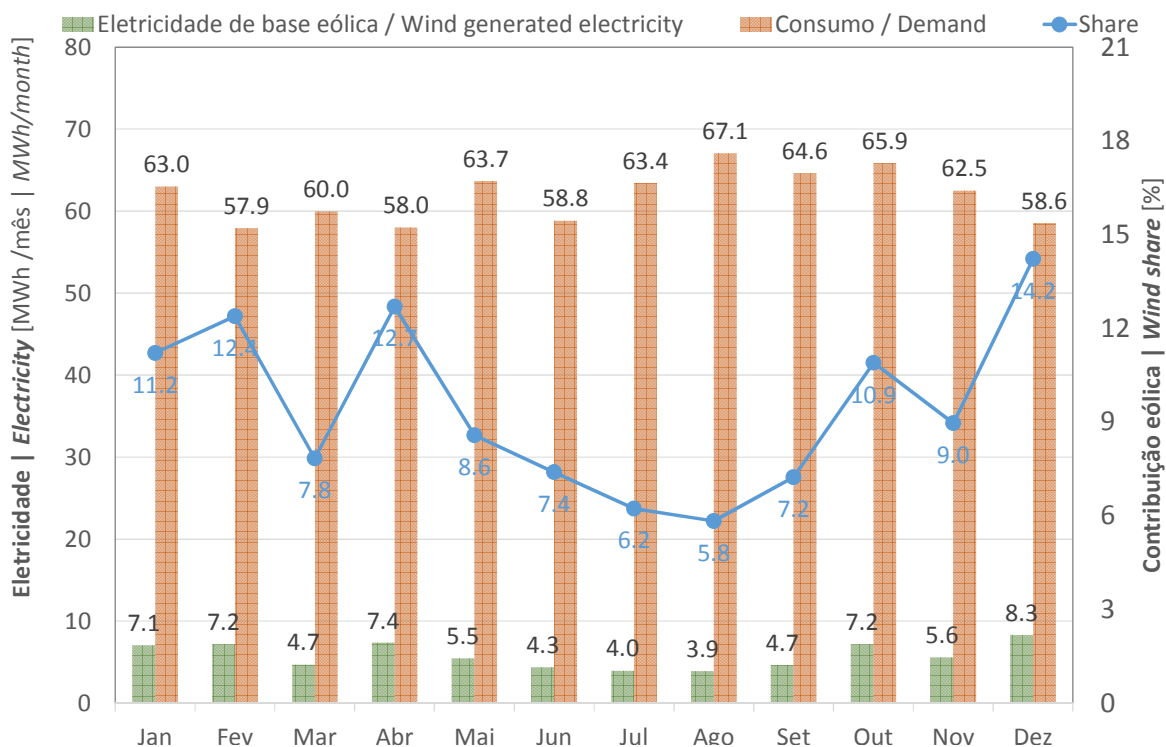
Figure 12: Wind generation vs. Electricity demand 2019 - Azores Autonomous Region
