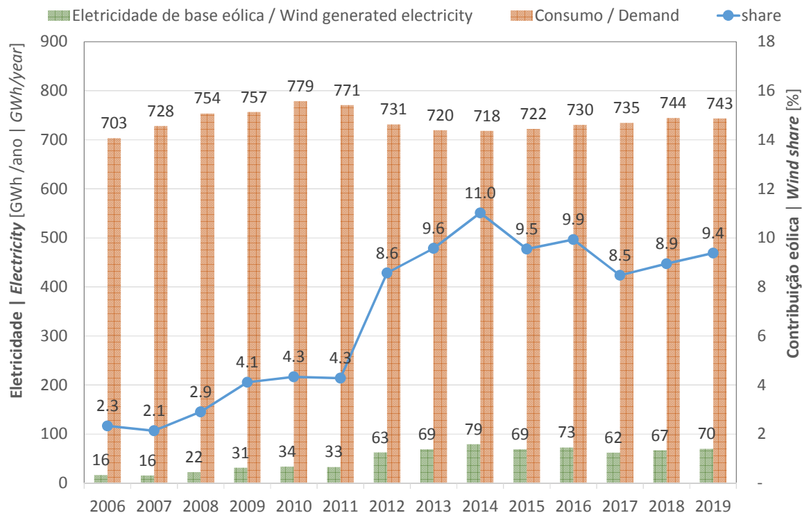
Figure 11: Wind generation vs. Electricity demand 2006-2019 - Azores Autonomous Region
