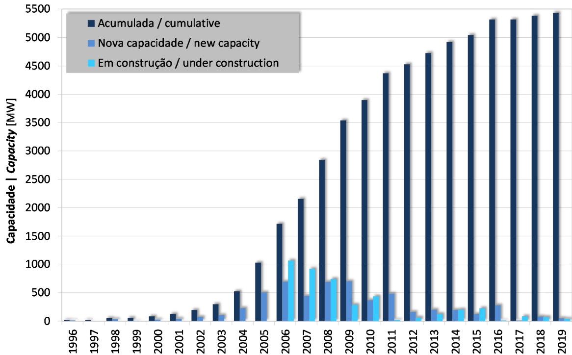
Figure 5: Cumulative installed capacity - Portugal
