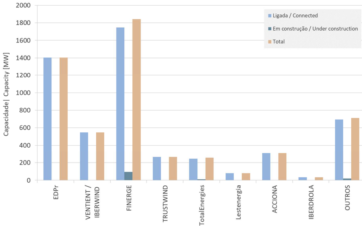
Figura 20: Promotores | 2023 Figure 20: Developers | 2023
