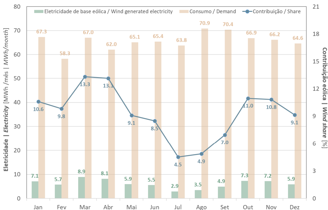
Figure 12: Wind generation vs. Electricity demand | 2023- Azores Autonomous Region
