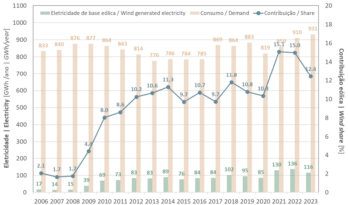
Figure 9: Wind generation vs. Electricity demand | 2006-2023 - Madeira Autonomous Region
