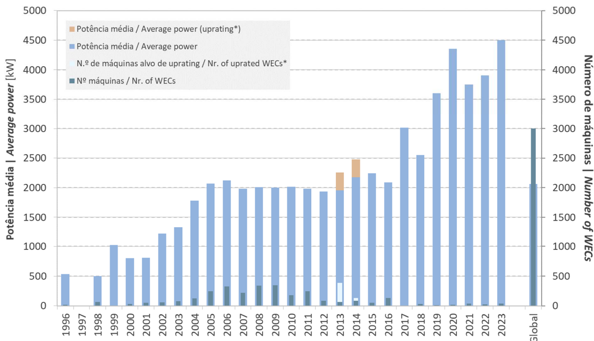
Figure 16: Number of WECs and average rated power 1996-2023
