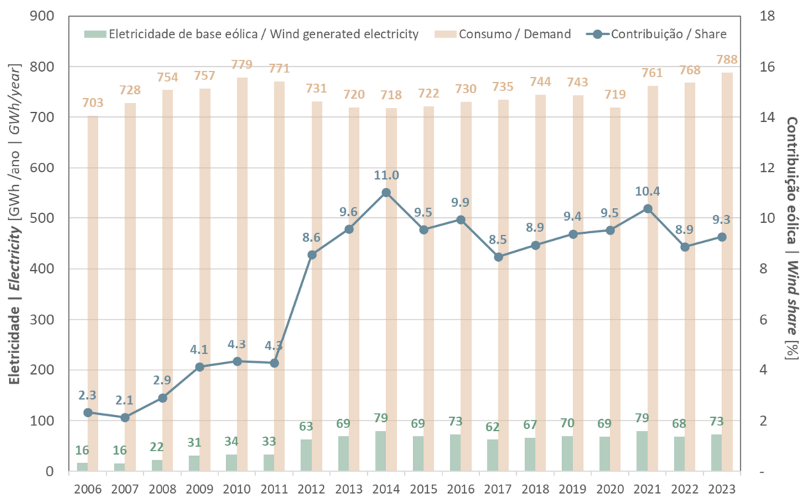
Figure 11: Wind generation vs. Electricity demand | 2006-2023 - Azores Autonomous Region
