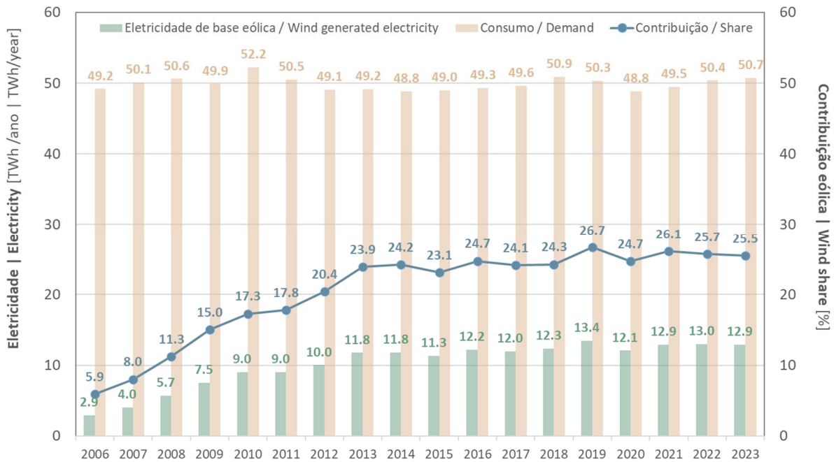
Figure 7: Wind generation vs. Electricity demand | 2006-2023 - Mainland Portugal 2
