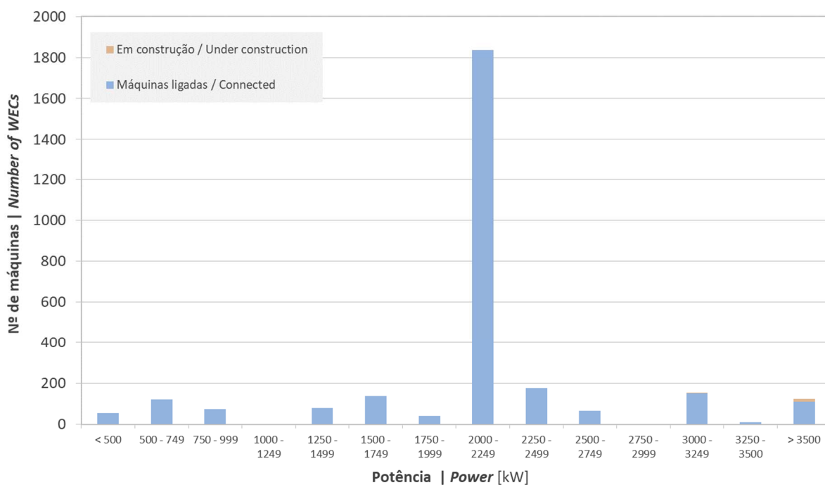
Figure 17: Number of WECs by power class | 2023
