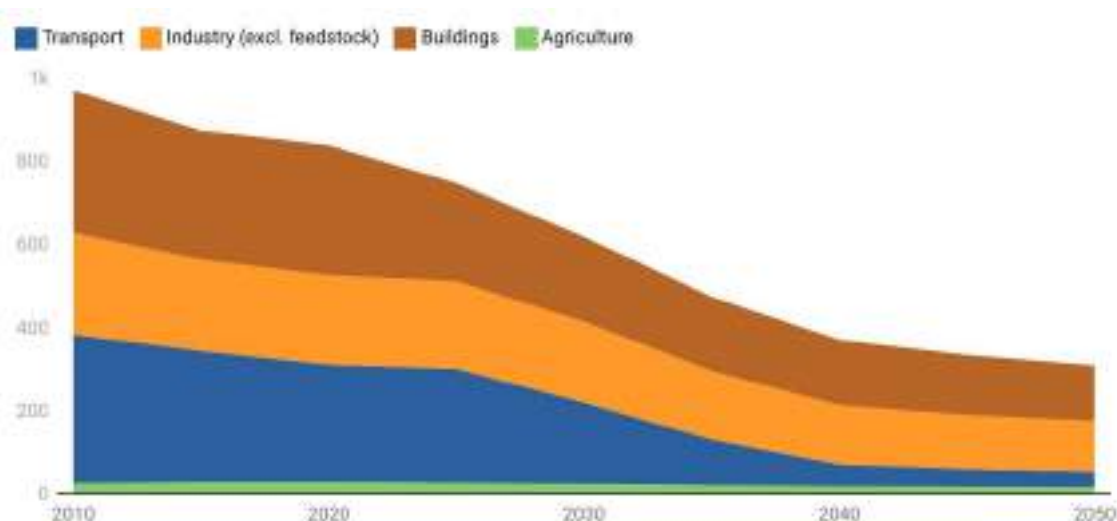
Figure 17 – Final energy consumption (TWh) by sector in Spain in the PAC scenario. Source: PAC scenario. Created with Datawrapper.
