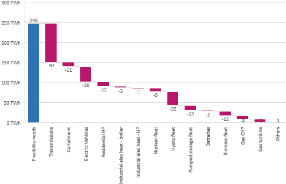
Figure 4-8: Contribution to remaining weekly flexibility needs per technology - Electrolyser contribution: 394 TWh
