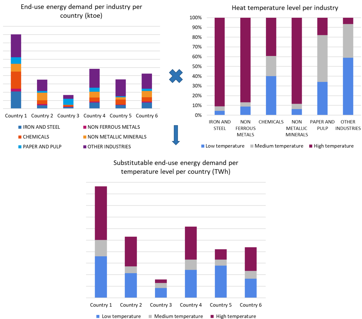
Figure 8-2: Methodology for the integration of industrial heat demand in the METIS model
