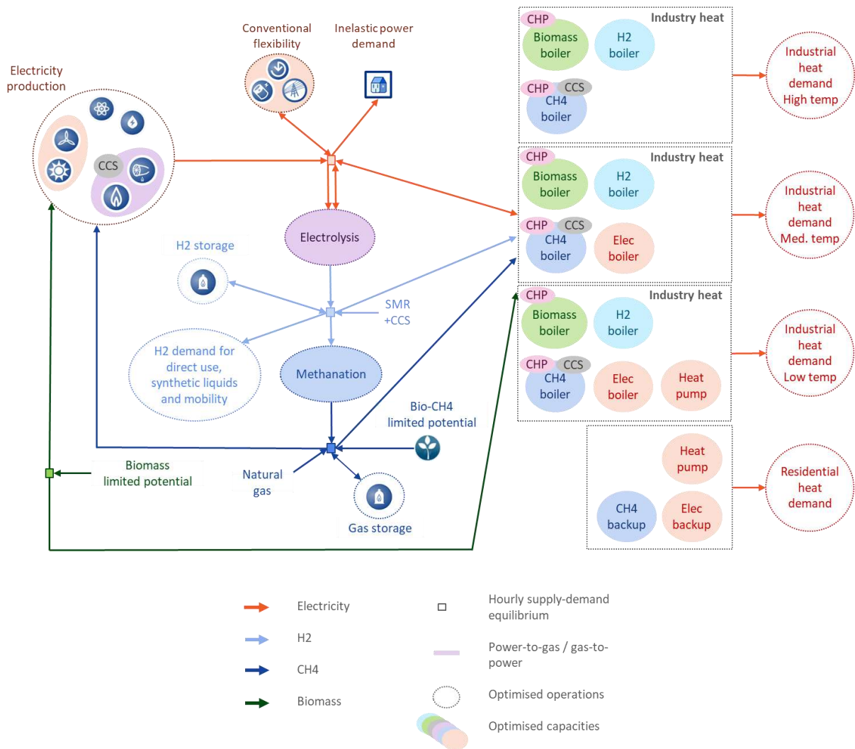
Figure 8-9: METIS multi-energy model used for the building of the METIS 1.5 scenario
