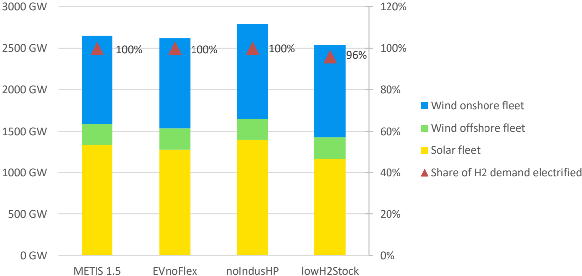
Figure 5-2: vRES installed capacities (EU27+7 scope)
