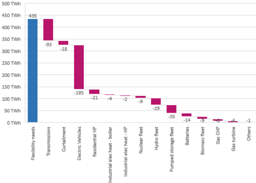
Figure 4-7: Contribution to remaining daily flexibility needs per technology - Electrolyser contribution: 516 TWh
