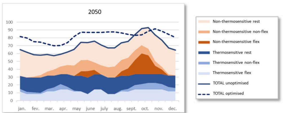
Figure 8-1: End-use decomposition of power demand
