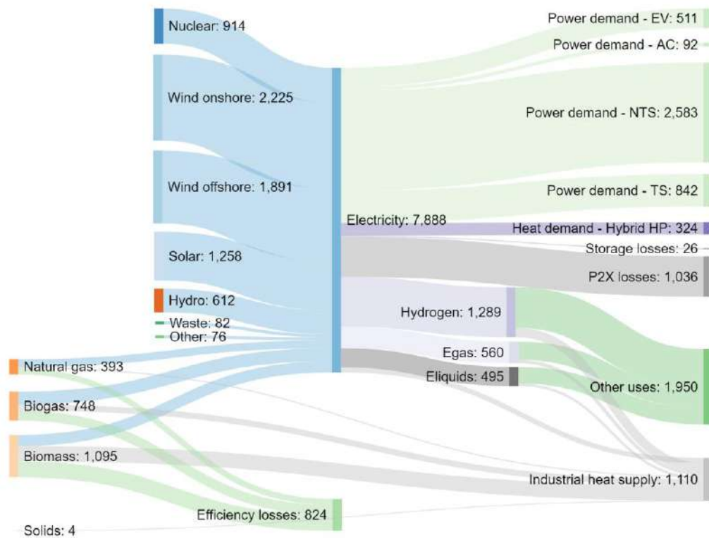
Figure 4-3: The European energy system in the 1.5TECH scenario (EU27+7) [TWh]
