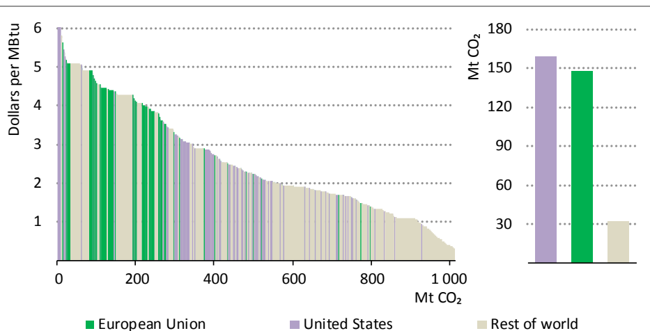
Figure 2.10 ▶ CO 2 emissions savings possible from coal-to-gas switching at different gas prices (left) and cost-effective savings in 2020 (right)
