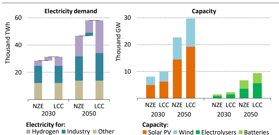
Figure 2.31 ▶ Impacts of achieving net-zero emissions by 2050 without expanded fossil fuel-based CCUS
