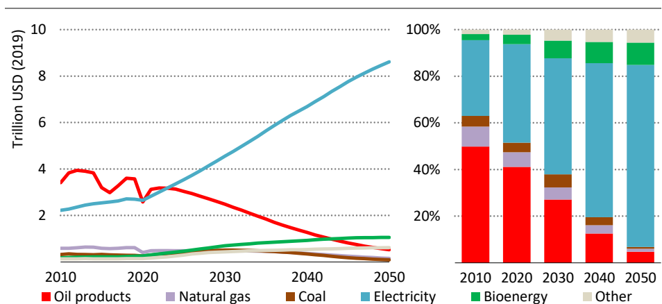
Figure 4.13 ▶ Global energy spending by fuel in the NZE
