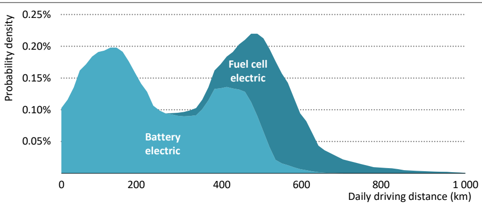
Figure 3.24 ▶ Heavy trucks distribution by daily driving distance, 2050
