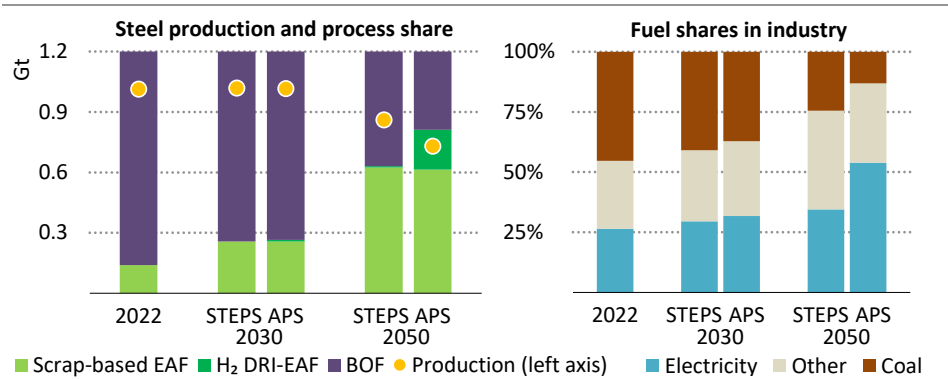
Figure 5.22 ▶ Steel production by process and fuel shares in industry in China by scenario, 2022-2050
