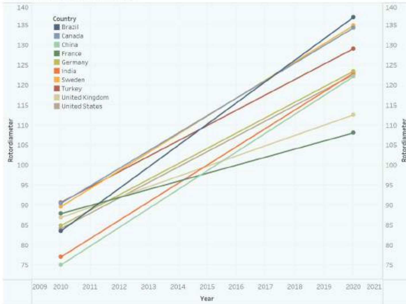
Rotor Diameter 2010-2020
