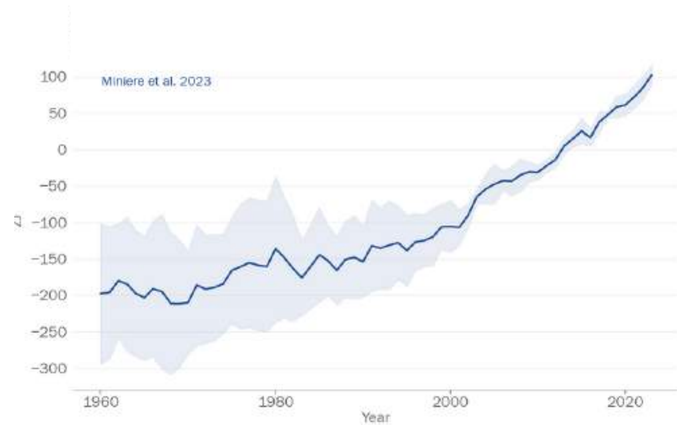
Figure 5: Ocean heat content from 1960-2023, shown as a difference from the 2005-2020 average: Source: Miniere et al. 2023.
