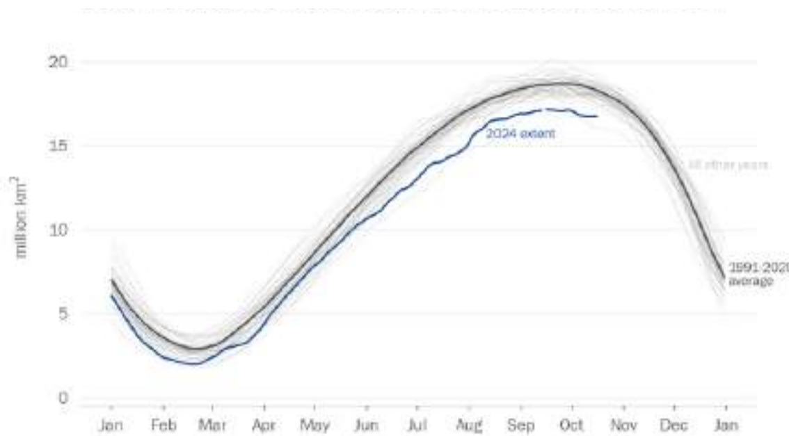
Figure 3: Daily Antarctic (top) and Arctic (bottom) sea ice extents in 2024 compared to the average and historical records since 1978. Source: National Snow and Ice Data Center
