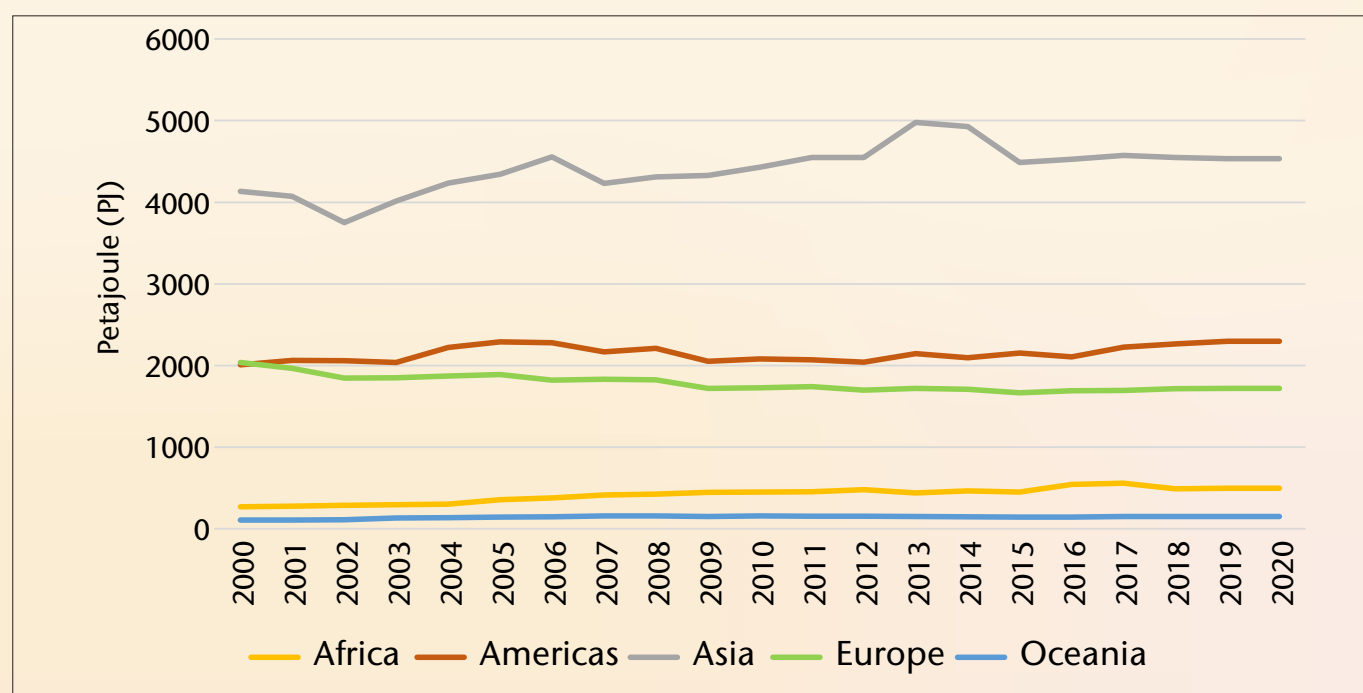
Figure 18. On-farm energy used (energy consumption) in agrifood systems, by region, 2000–2020 Source: Data from the Food and Agriculture Organization Corporate Statistical Database, FAOSTAT
